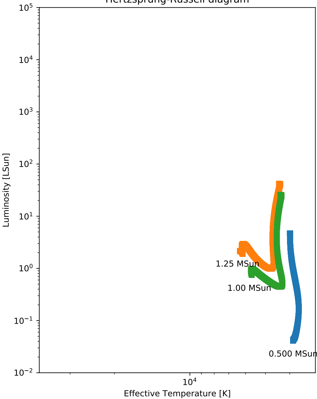
Hertzprung-Russell diagram
